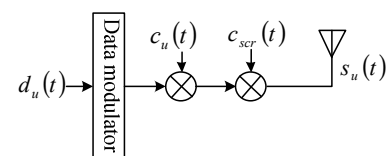
(a). Transmitter
