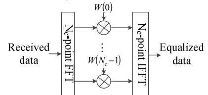
Figure 7. Frequency domain equalizer
