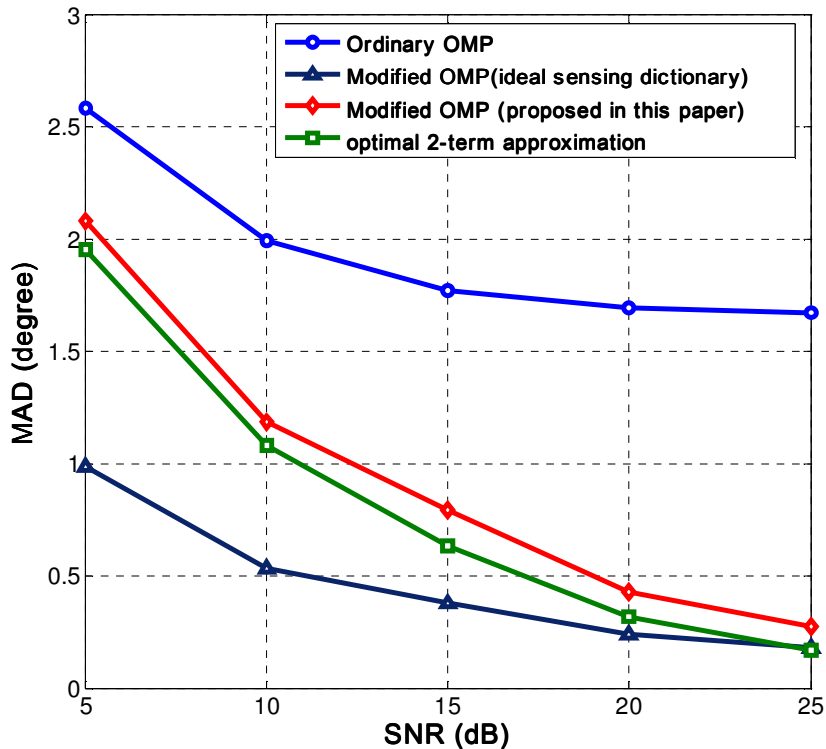
Figure 2. MAD via SNR for estimation of DOA 2 =17°.
