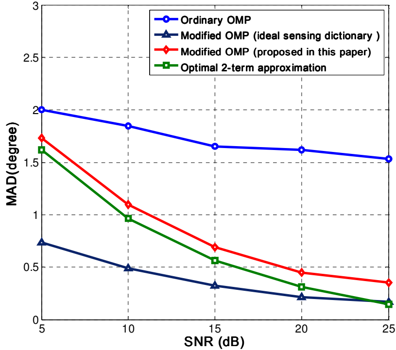
Figure 1. MAD via SNR for estimation of DOA1=8°.
