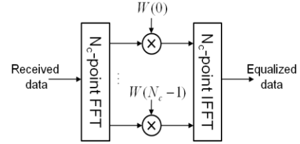
Fig.7 Frequency domain equalizer
