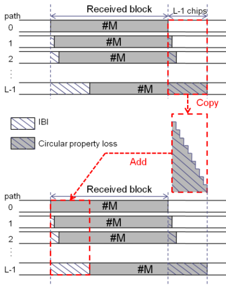
Fig. 6 Imperfect circular property loss restoration
