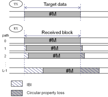
Fig.2 IBI and Circular property loss
