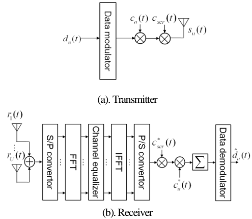
Fig.1 System model of the multi-code DS-CDMA
