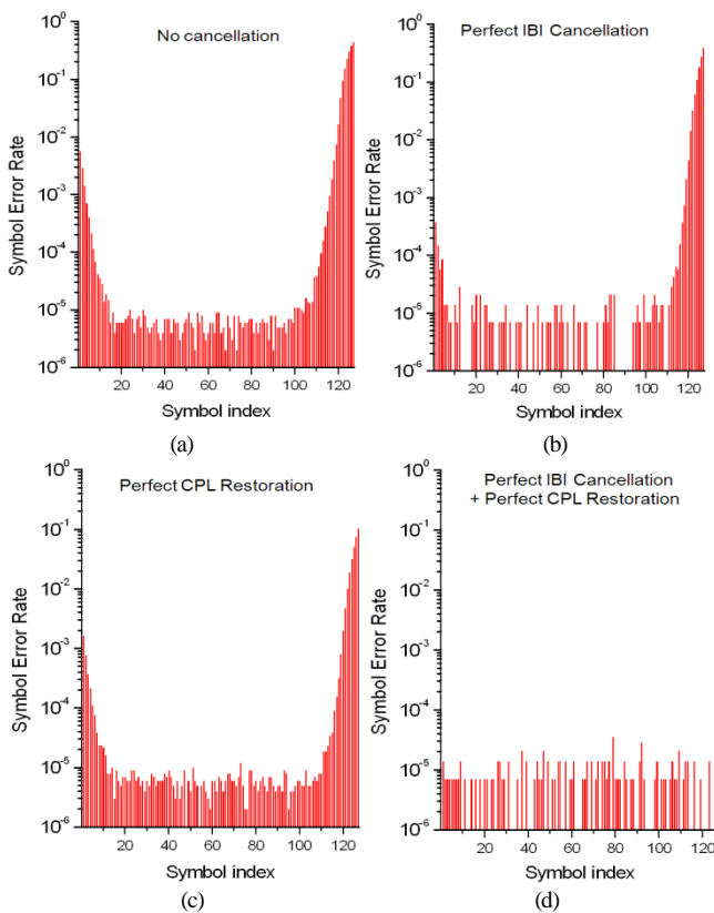
Fig. 9 Distribution of symbol error rate
