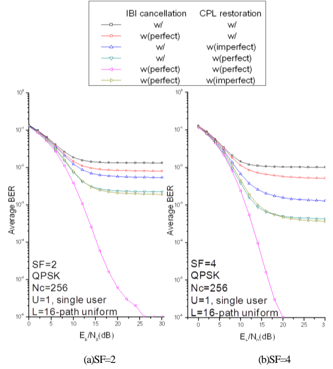
Fig. 8 Average BER performance comparison
