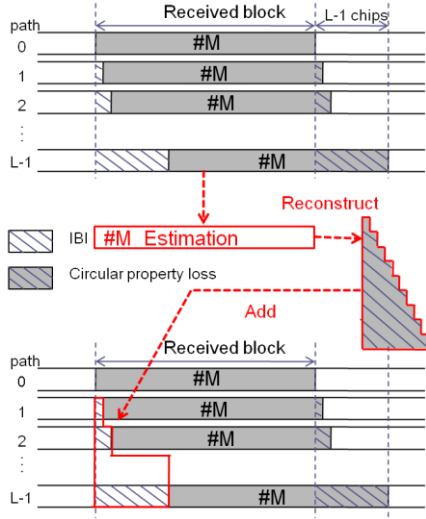
Fig. 5 Perfect circular property loss restoration
