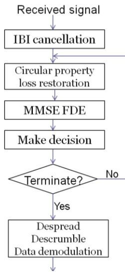
Fig. 3 Flow at receiver side
