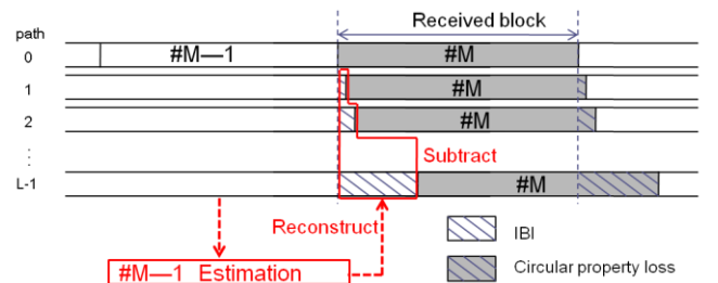
Fig. 4 Perfect IBI cancellation
